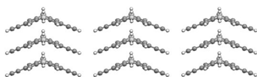
Figure 1. Structure of an ab plane formed by stacks of the bent molecule 2 .
